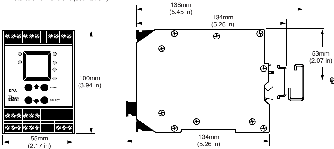
Figure 13. Installation dimensions (see Table 2).
