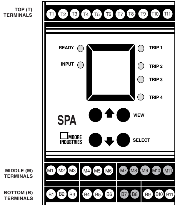
Figure 15. Terminal position and sensor hook-up guides.
