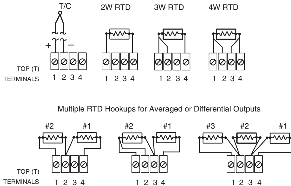
Figure 16. Temperature sensor hook-up guide for TPRG units.
