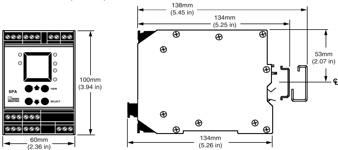
Figure 14. Installation dimensions (see Table 2).
