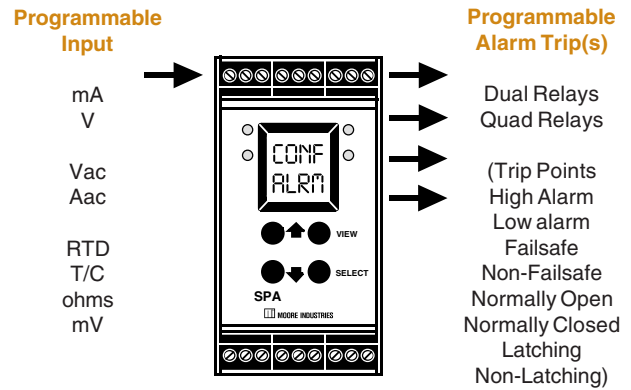
Figure 1. Available models deliver versatile input/output choices.
