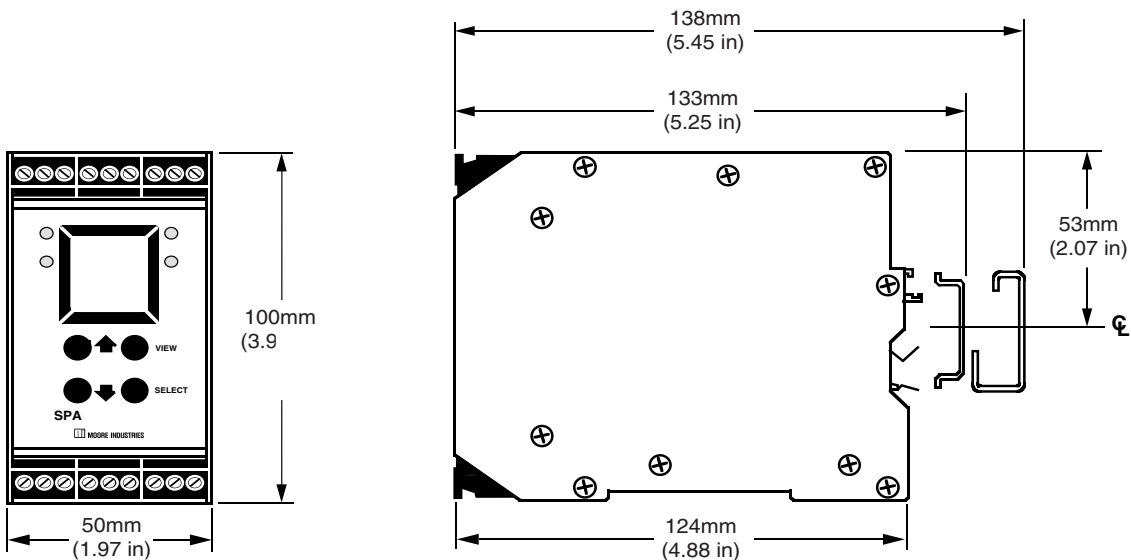
Figure 11. Installation dimensions (see Table 2).
